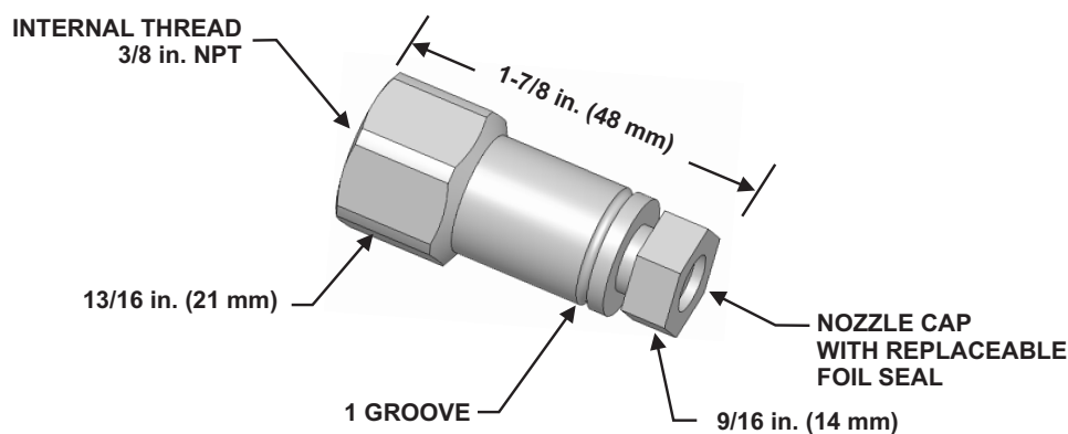
Figure 1. ADP Nozzle
