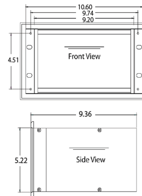
8800 Controller Rack/Panel Mount (19" Rack Spreader Plates Not Shown)
