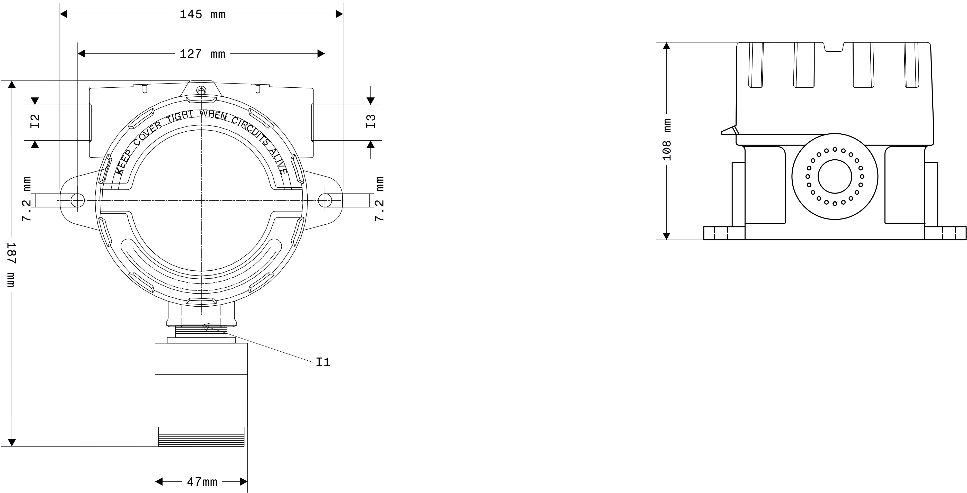
Mechanical drawings SMART S-SS with 4A enclosure
