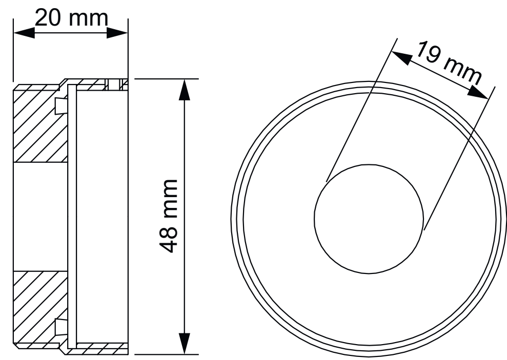
STG/AD3 dust adapter
