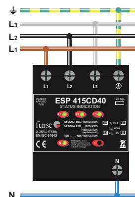
Parallel connection of ESP 415CD40 to three phase supplies (fuses not shown for clarity)
