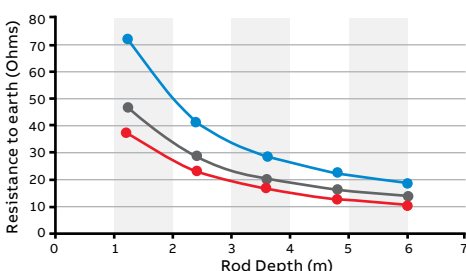
Rod only Ø 100mm backfill Ø 200mm backfill Note: Based on 100 Ohm metre soil
