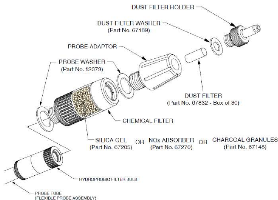
Figure 45: Filter Removal
