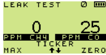
Figure 18: Methane + CO
