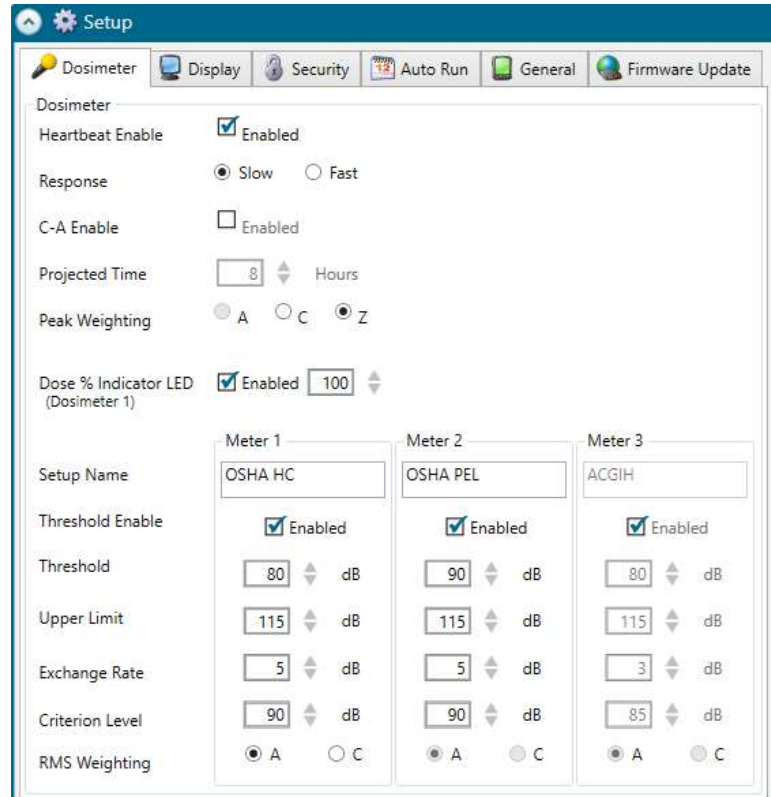
Figure 1-3 Parameter Setup Screen for EG-4P
