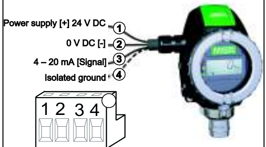
3-wire connection - PrimaX P
