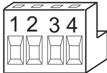
Fig. 3 Terminal PrimaX P (3-wire sensor)
