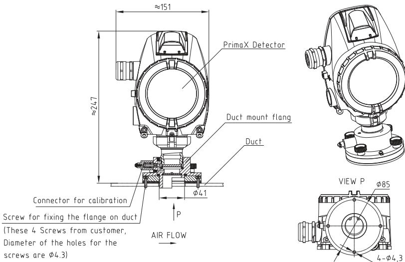
Fig. 29 Duct mounting
