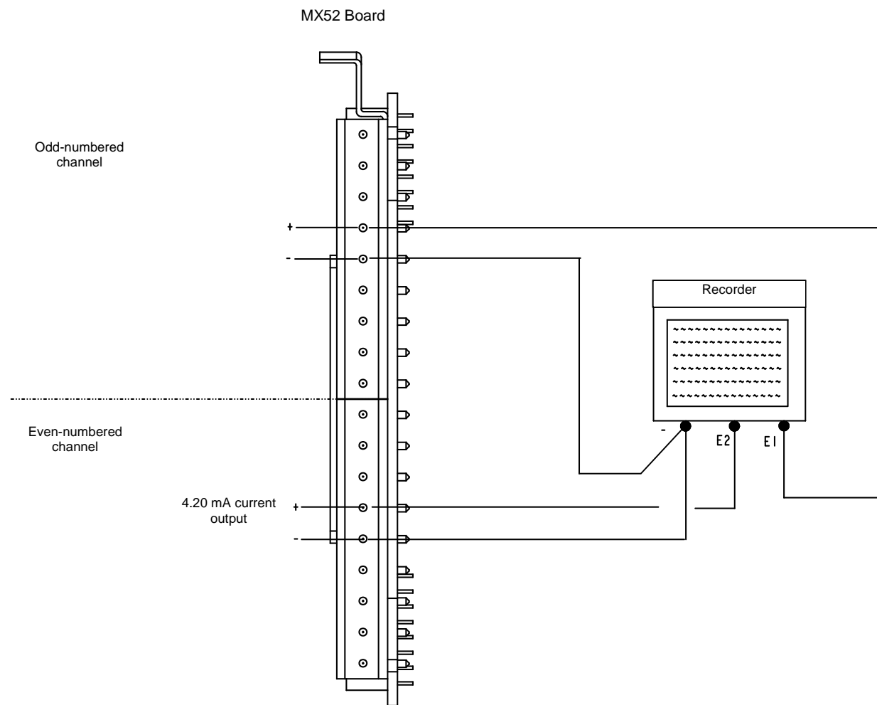
EXAMPLE OF CONNECTION OF A RECORDER TO THE 4-20 OUTPUT OF A MEASURING CHANNEL
