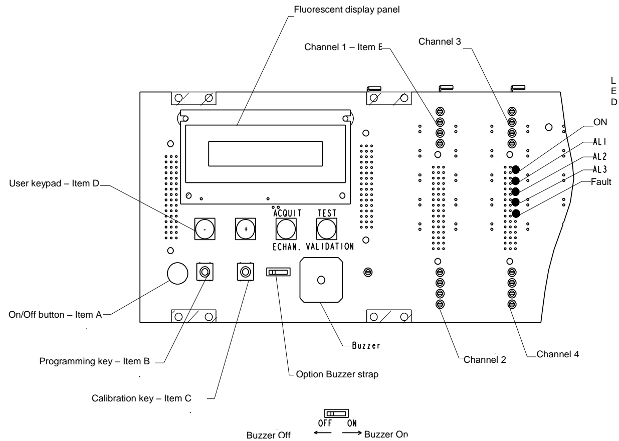
MAIN OPERATING COMPONENTS
