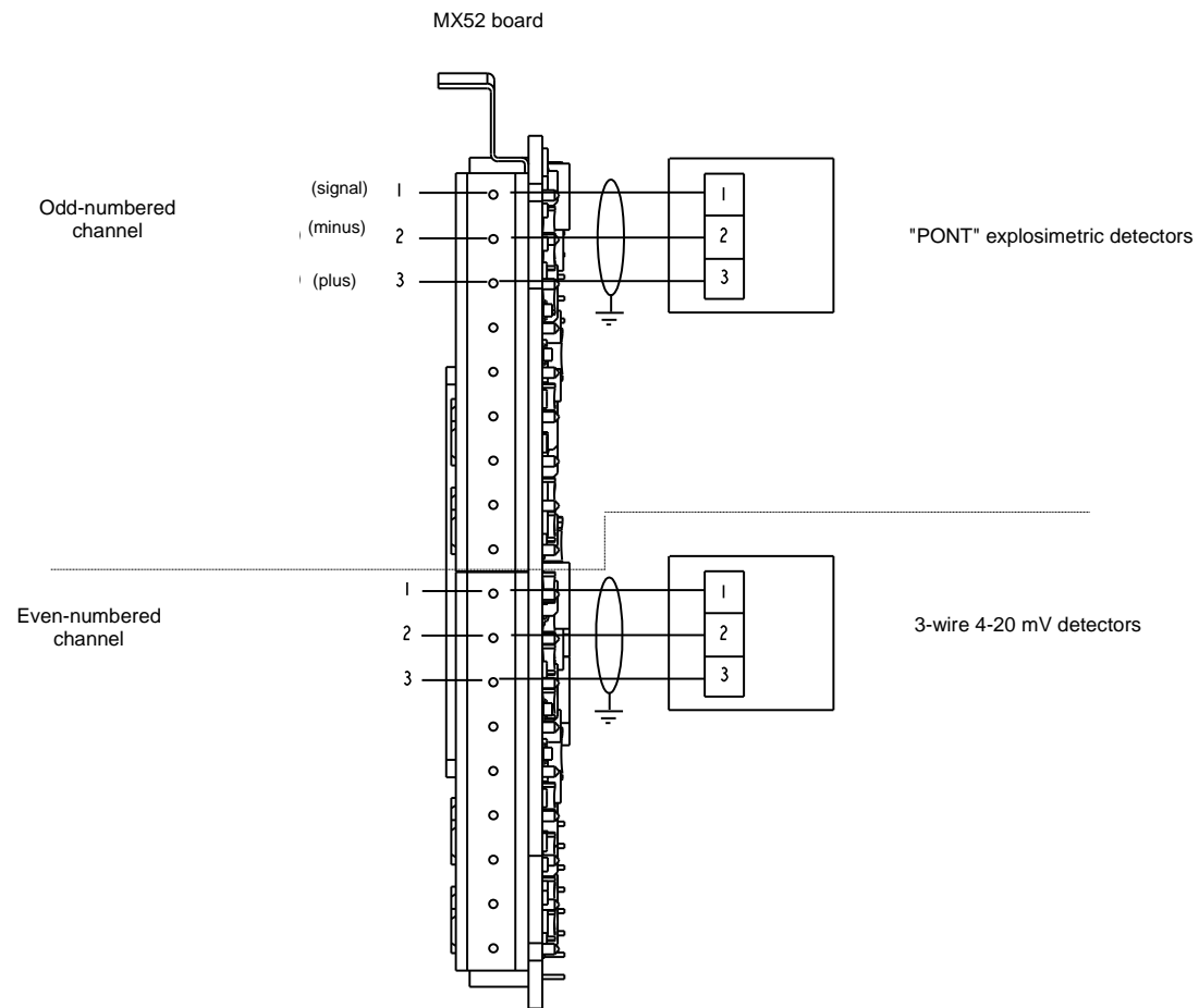
EXAMPLE OF CONNECTION OF EXPLOSIMETRIC DETECTORS AND 3-WIRE 4-20 mA DETECTORS ON MX52
