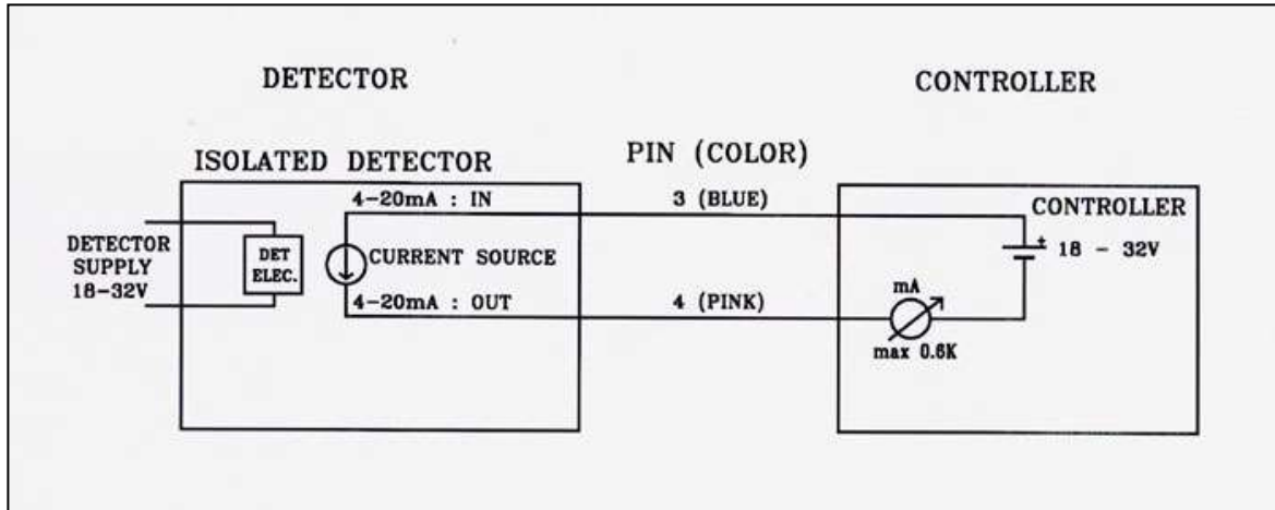
Figure 13: 4-20mA Wiring (Sink Option)
