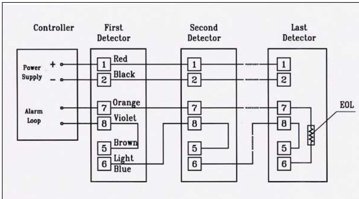
Figure 15: Typical Wiring for 4 Wire Controllers
