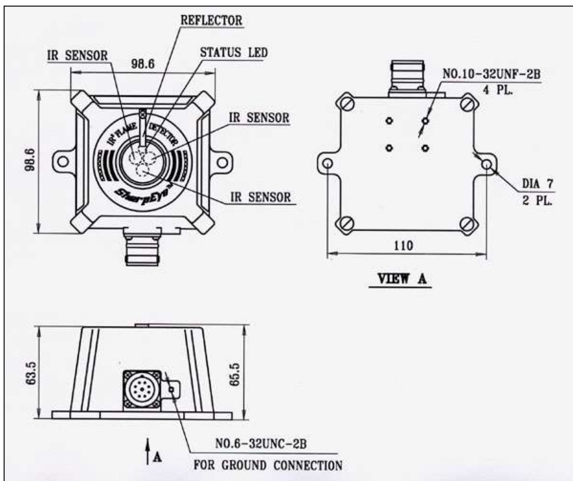
Figure 3: Flame Detector Assembly - Outline Drawing (Connector Output Option)
