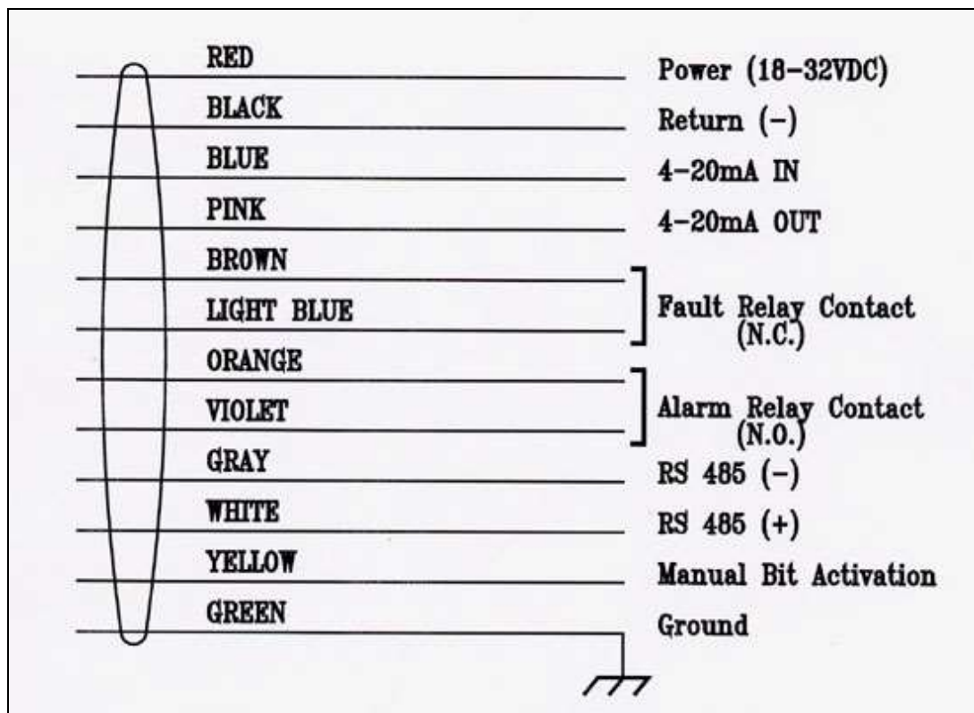
Figure 11: Cable Interface Option
