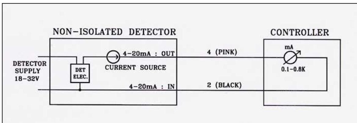
Figure 14: 4-20mA Wiring (Source Option)
