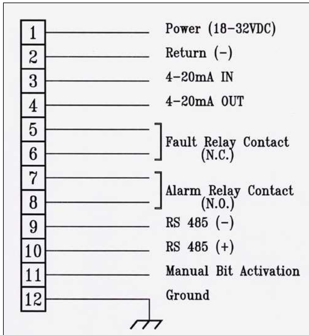
Figure 10: Connector Interface Option
