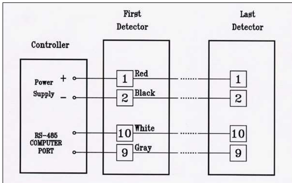
Figure 12: RS-485 Networking
