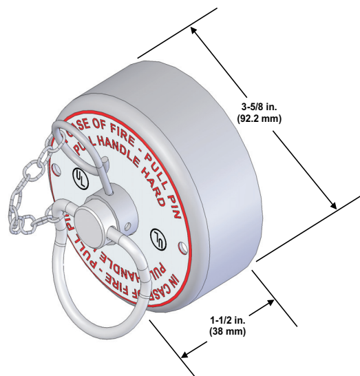
Figure 1. Mechanical Remote Manual Release, P/N WK-875572-000
