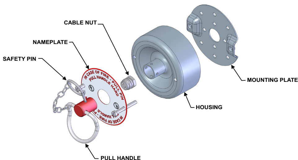
Figure 2. Exploded View
